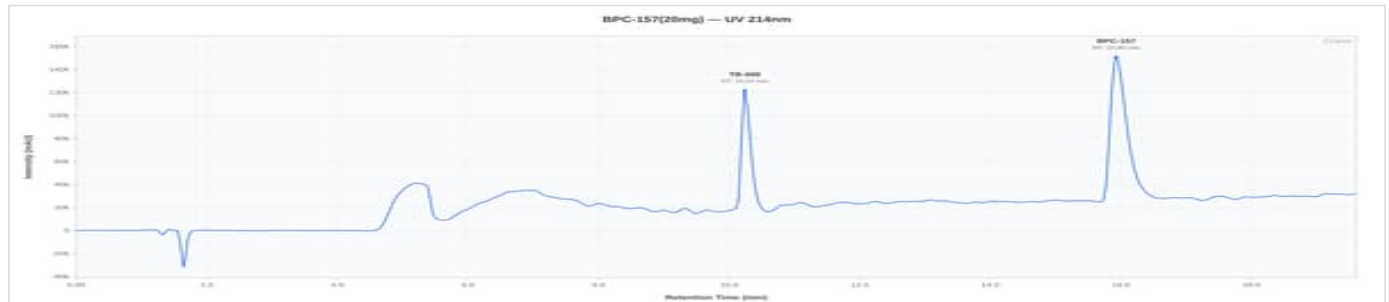
BPC-157/TB-500 Wolverine 20mg - EB-BB20-01: UV Chromatogram
